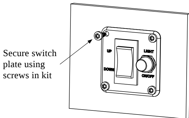
Figure 20. Securing switch plate to winch cover
