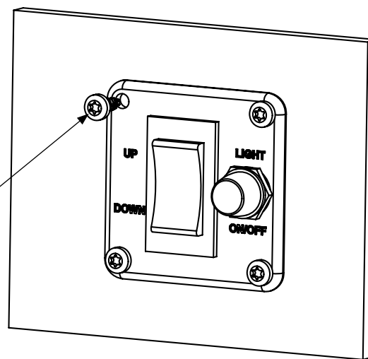
Figure 17. Securing switch plate to helm
